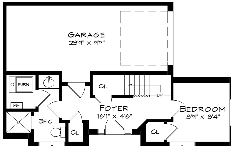
GROUND LEVEL 354 SQUARE FEET + 265 SF (GARAGE)
